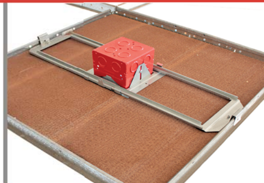
Ceiling T-Bar
