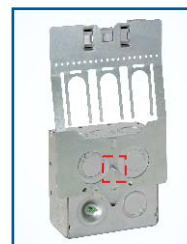
Installed with just one Tek Screw
