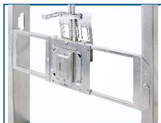
BMCS-CJ6 installed on SSB Bracket helps minimize the field work
