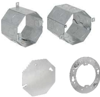
CONCRETE BOXES & RINGS
